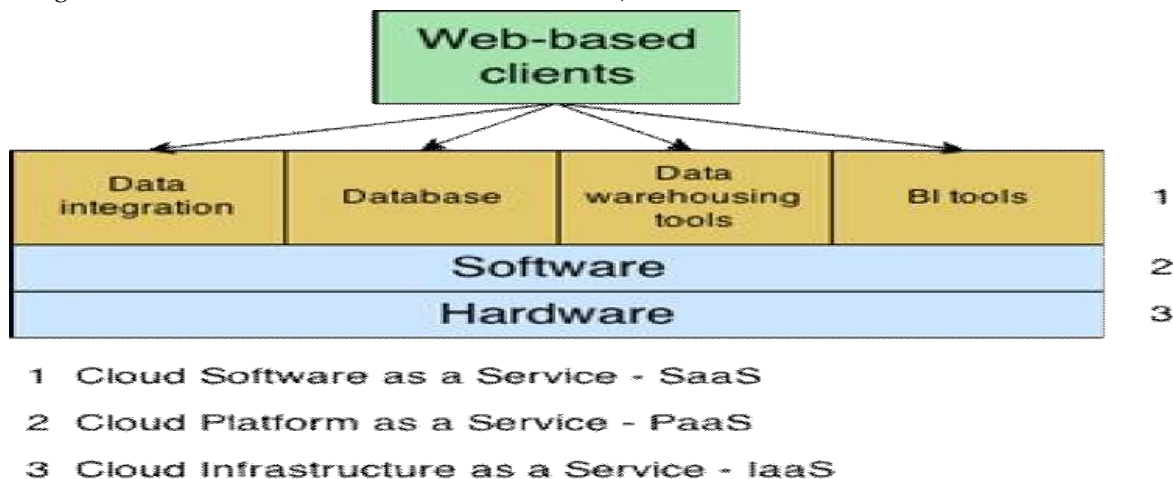
Fig. 6. Cloud BI or integrating Business Intelligence solutions into Cloud -> Basic Architecture [6]
