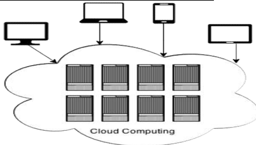
Fig. 2. Cloud Computing
